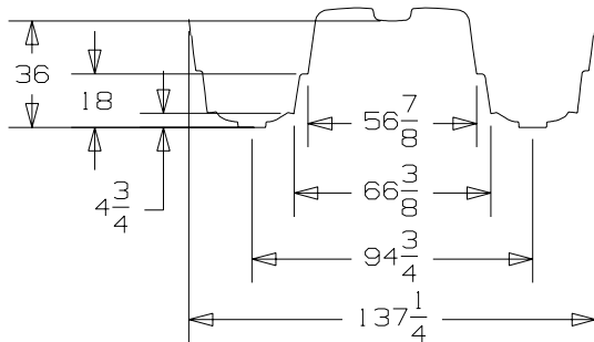
SECTION AT TRANSOM
