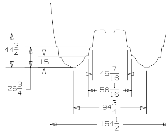
SECTION AT MIDSHIP
